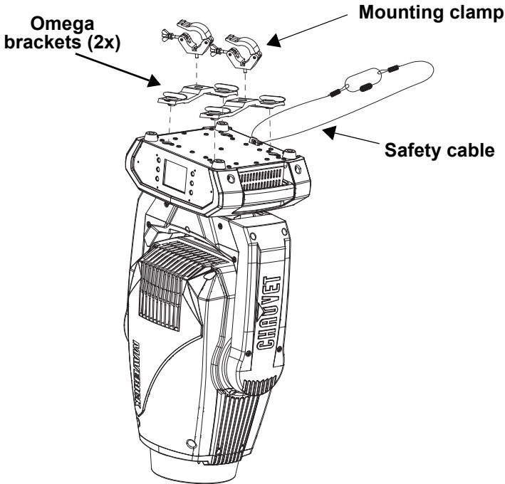
Overhead Mounting
