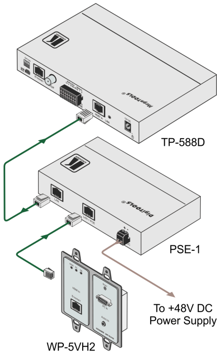
Figure 3: Connecting the PSE-1 10G POE Injector
