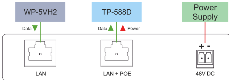
Figure 4: Alternative Connection for the PSE-1 10G POE Injector
