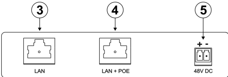
Figure 2: PSE-1 10G POE Injector Rear Panel
