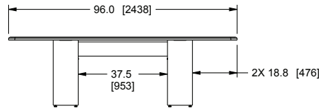
8' KLASIK SIDE VIEW
