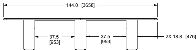
12' KLASIK SIDE VIEW
