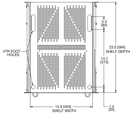
TOP VIEW (SHELF NOT EXTENDED)
