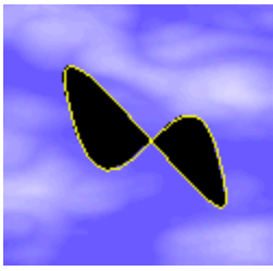
Bézier Mask
