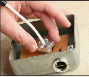
Fig D. Install the threaded nut with shoulder side down and secure.
