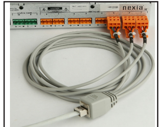
Fig L. Connect RJ45 cables into the breakout cable and connect to DSP Controller.
