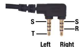
3.5 mm Dual Mini (Gold) TRRS Connector
