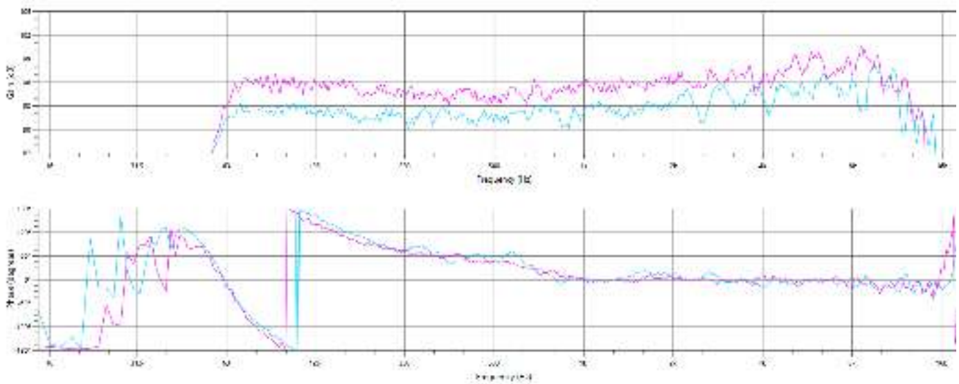
Figure 22: LEO (magenta) and LYON (blue) Loudspeaker Phase Responses-with pc100 Delay Integration
