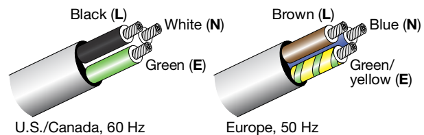
Figure 8: AC Wiring Scheme, illustrated
