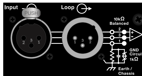
Figure 11: XLR 3-Pin Audio Connectors, Input and Loop Output
