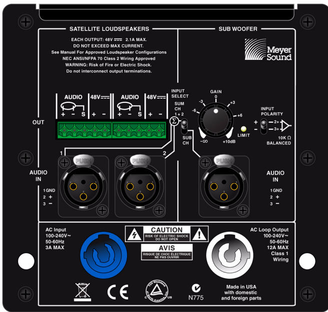
MM-10ACX Rear Panel, Shown with Phoenix Satellite Connectors
