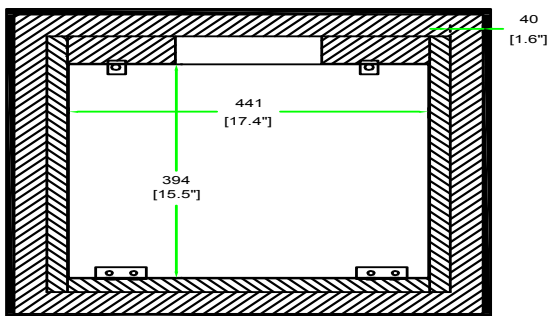
TOP VIEW OF COVER
