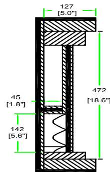
B-B VIEW
