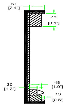
D-D VIEW
