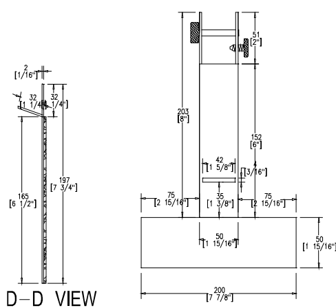
FRONT VIEW OF STAND
