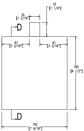
TOP VIEW OF RRSER
