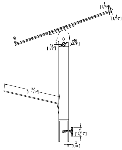
SIDE VIEW OF TRAY
