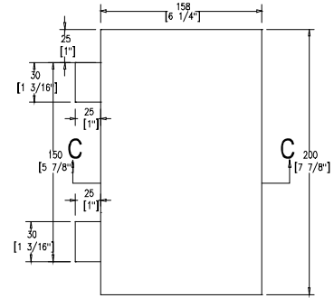
C-C VIEW
