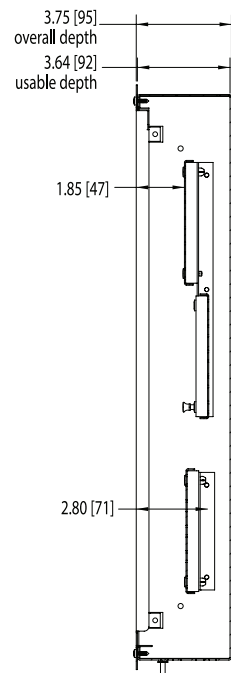
SIDE SECTION with trim ring
