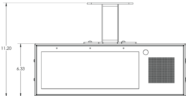
Ceiling Mount Front
