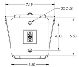
Ceiling Mount Side
