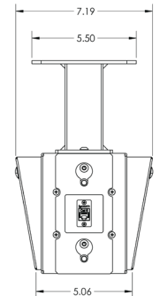
Ceiling Mount Side
