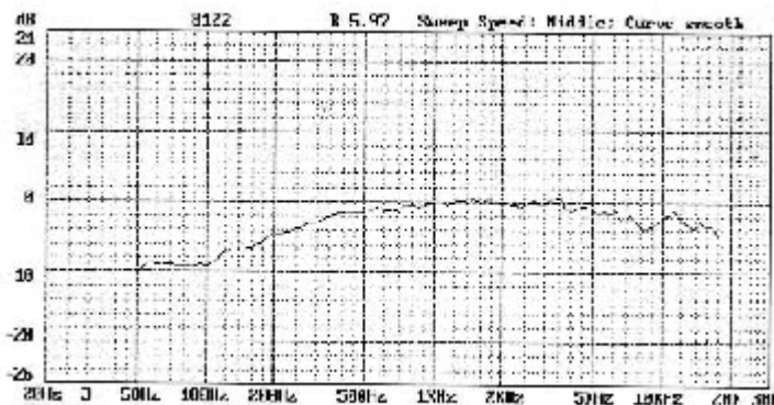
Frequency Response Curve
