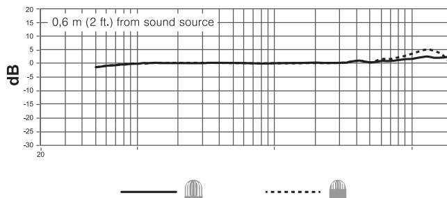
Frequency Response
