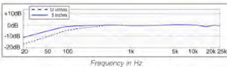
Frequency Response of SR25 (typical)
